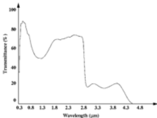
Figure 4. Transmittance diagram of a typical side window.
