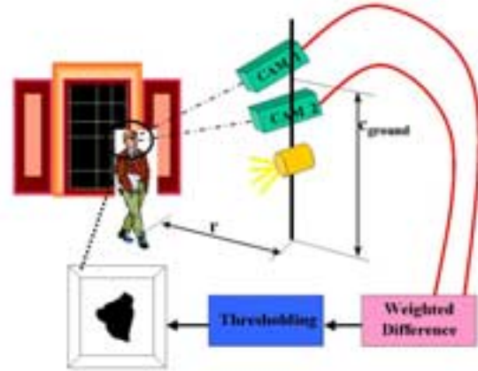
Figure 6. Architecture of the dual-band face detection system.
