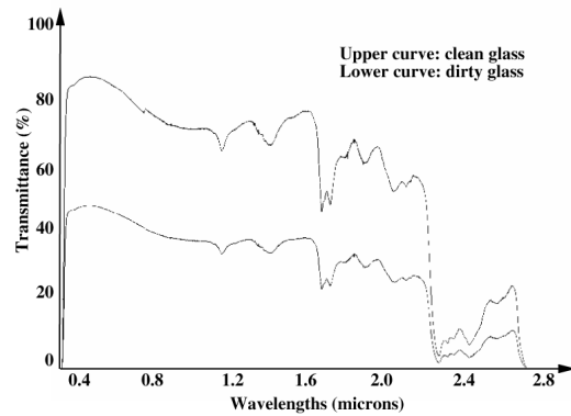
Figure 5. Transmittance diagram of a typical windshield.
